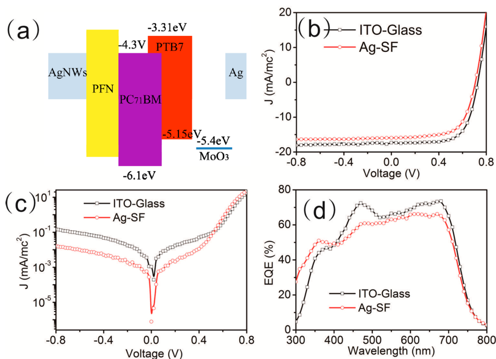
Figure 4. (a) Energy band diagram of the device. (b) J - V curves of the OSCs fabricated on ITO different substrates under AM 1.5G and light intensity of 100 \text{ mW/cm}^2 . (c) J - V curves of the OSCs in the dark. (d) Corresponding EQE curves of OSCs on AgNW/SF and ITO glass substrate.
